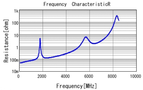
■ GQM1885C1H560JB01 R DCOV, 25degC
