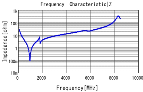
■ GQM1885C1H560JB01 |Z| DCOV, 25degC
