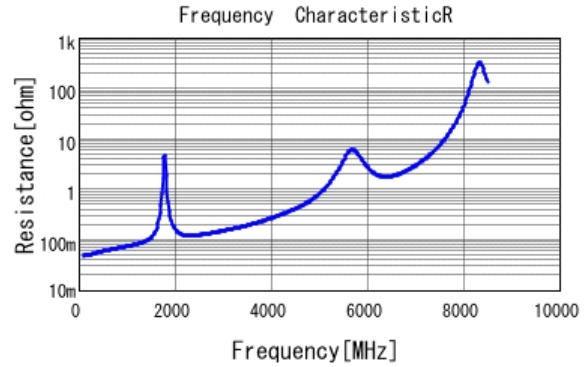
■ GQM1885C1H560GB01 R DCOV, 25degC
