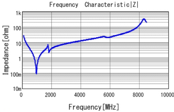
■ GQM1885C1H560GB01 |Z| DCOV, 25degC
