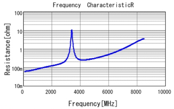
■ GQM1885C1H150JB01 R DCOV, 25degC
