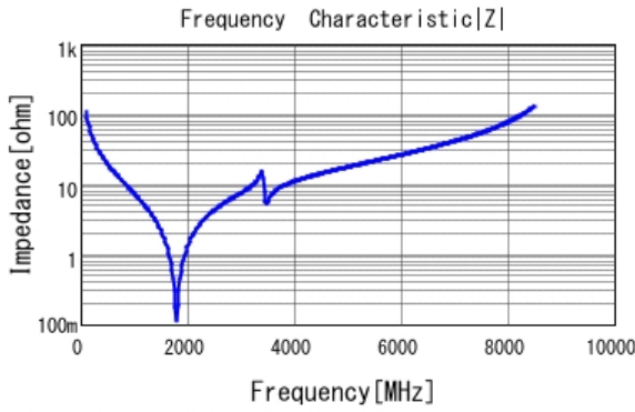
■ GQM1885C1H150JB01 |Z| DCOV, 25degC
