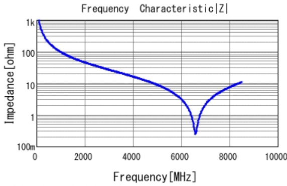
■ GQM1875C2E1R6BB12 |Z| DCOV, 25degC
