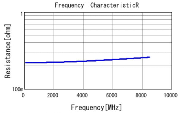
■ GQM1875C2E1R6BB12 R DCOV, 25degC
