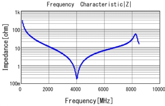
■ GQM1555C2D5R6CB01 |Z| DCOV, 25degC
