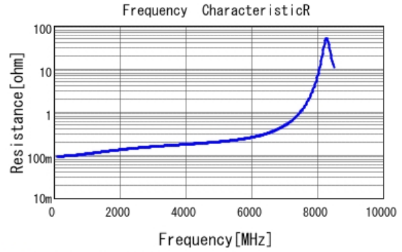
■ GQM1555C2D5R6CB01 R DCOV, 25degC
