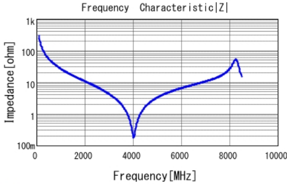
■ GQM1555C2D5R6BB01 |Z| DC0V, 25degC
