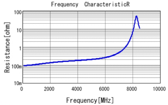
■ GQM1555C2D5R6BB01 R DC0V, 25degC
