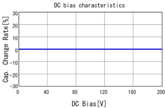
■ GQM1555C2D5R6BB01 C-DC bias capchange, 25.0degC, AC1V
