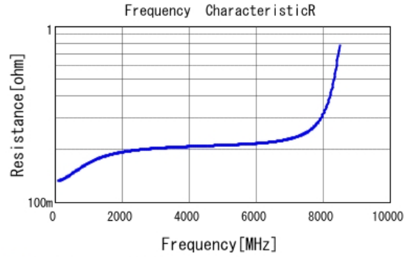
■ GQM1555C2D1R6CB01 R DC0V, 25degC
