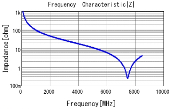
■ GQM1555C2D1R6CB01 |Z| DC0V, 25degC
