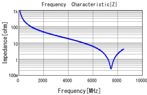
■ GQM1555C2D1R6BB01 |Z| DC0V, 25degC
