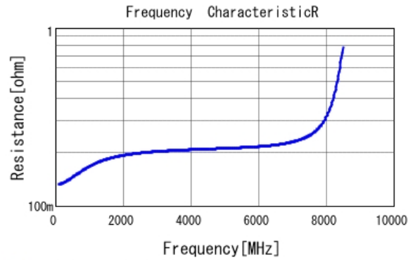
■ GQM1555C2D1R6BB01 R DC0V, 25degC
