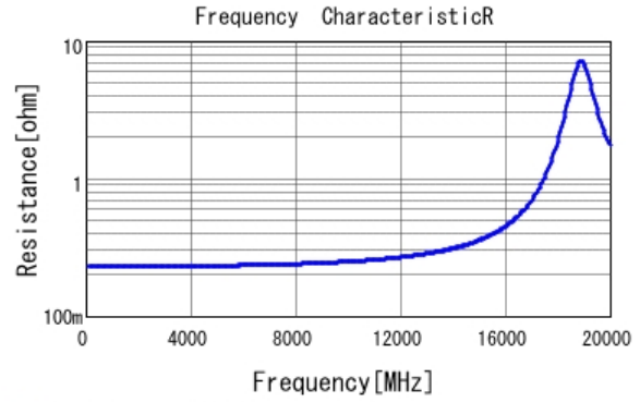
■ GQM1555C2D1R0BB01 R DC0V, 25degC
