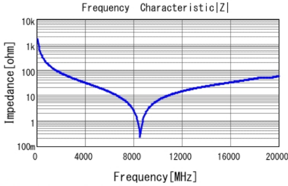
■ GQM1555C2D1R0BB01 |Z| DC0V, 25degC
