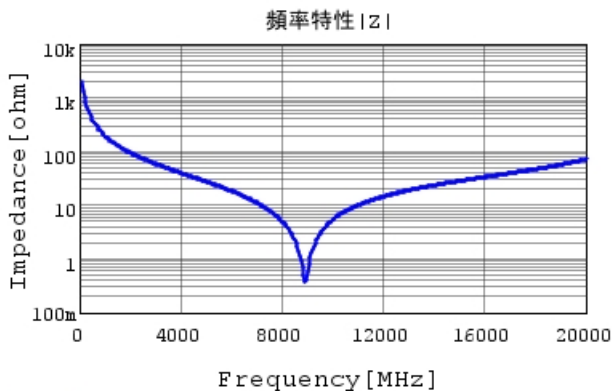
GJM1555C1HR80WB01 |Z| DCOV, 25degC
