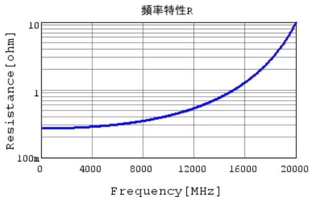
GJM1555C1HR80WB01 R DCOV, 25degC
