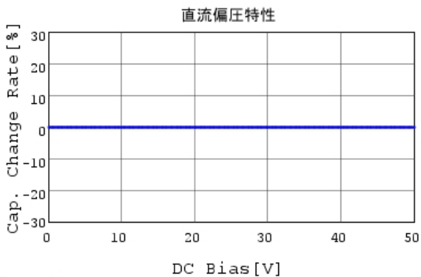
GJM1555C1HR80WB01 C-DC bias capchange, 25.0c
