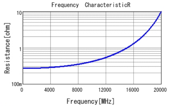
■ GJM1555C1HR80BB01 R DC0V, 25degC
