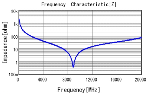
■ GJM1555C1HR80BB01 |Z| DC0V, 25degC
