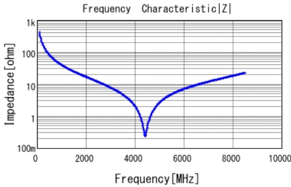
■ GJM1555C1H3R8BB01 |Z| DC0V, 25degC
