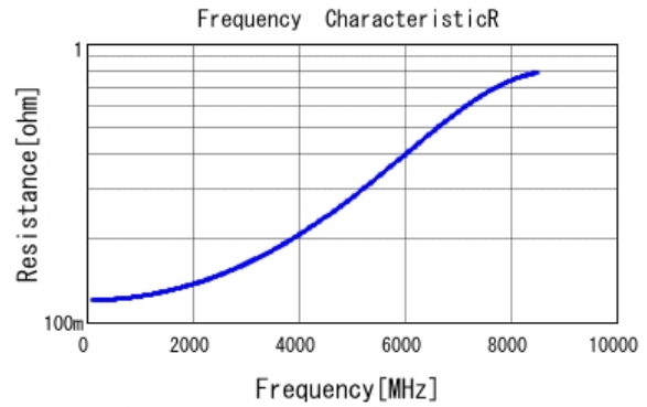
■ GJM1555C1H3R8BB01 R DC0V, 25degC
