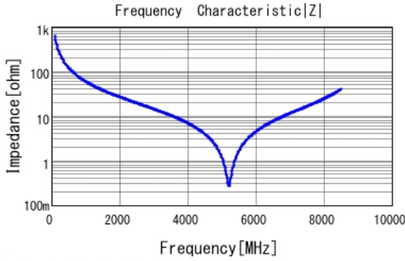
■ GJM1555C1H2R6BB01 |Z| DC0V, 25degC
