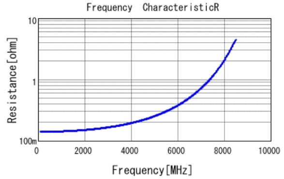
■ GJM1555C1H2R6BB01 R DC0V, 25degC
