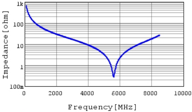
GJM1555C1H2R4CB01 |Z| DCOV, 25degC
