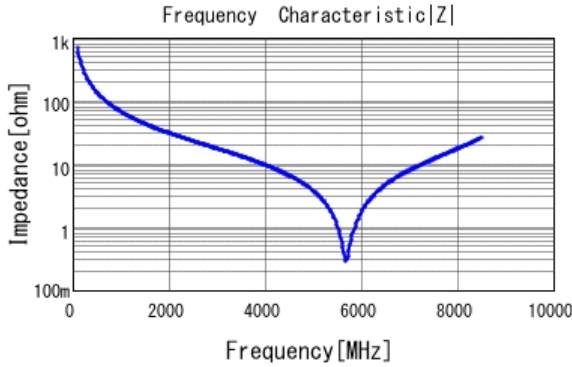
■ GJM1555C1H2R3WB01 |Z| DCOV, 25degC
