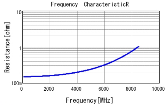
■ GJM1555C1H2R3WB01 R DCOV, 25degC
