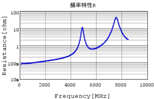
GJM1555C1H180GB01 R DCOV, 25degC
