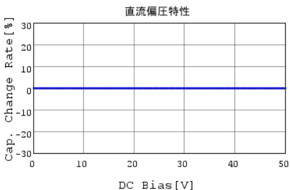
GJM0335C1HR80WB01 C-DC bias capchange, 25.0c
