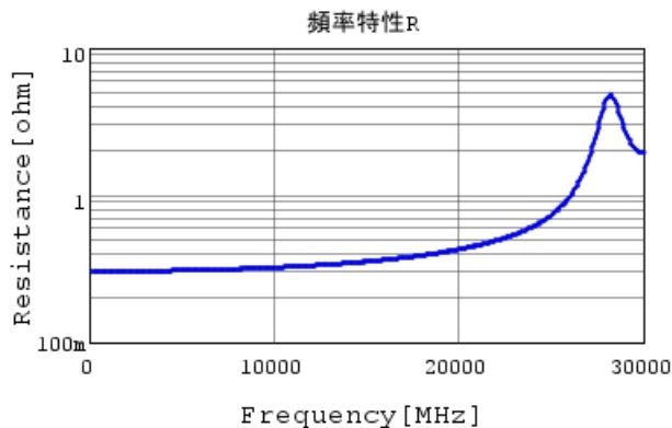
GJM0335C1HR80WB01 R DCOV, 25degC
