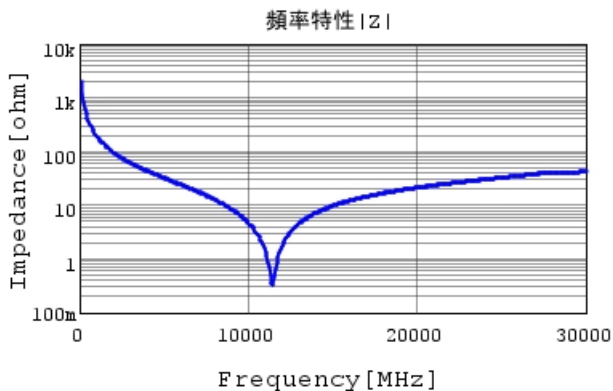
GJM0335C1HR80WB01 |Z| DCOV, 25degC
