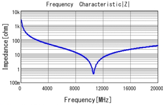
■ GJM0335C1ER70WB01 |Z| DCOV, 25degC
