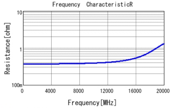
■ GJM0335C1ER70WB01 R DCOV, 25degC
