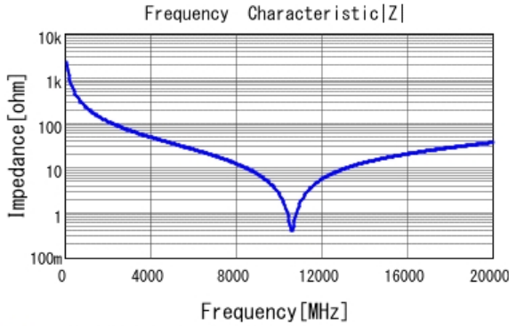
■ GJM0335C1ER70BB01 |Z| DC0V, 25degC
