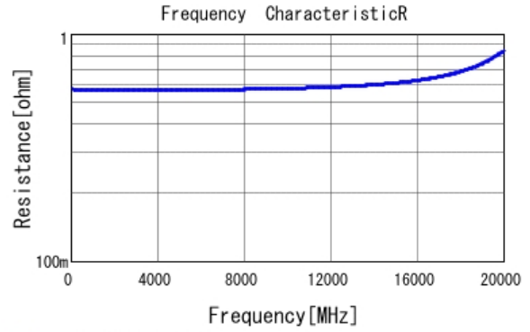
■ GJM0335C1ER20WB01 R DCOV, 25degC
