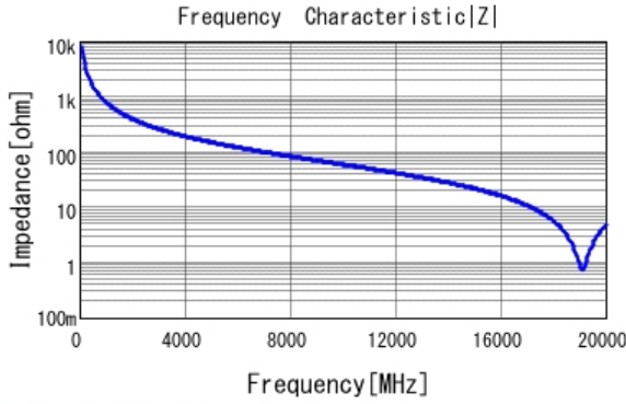
■ GJM0335C1ER20WB01 |Z| DCOV, 25degC
