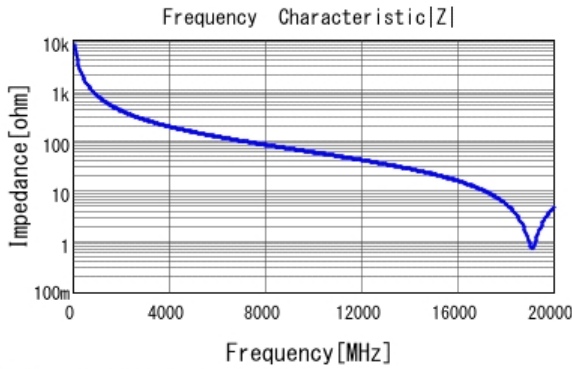
■ GJM0335C1ER20BB01 |Z| DC0V, 25degC
