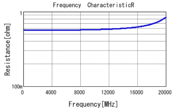
■ GJM0335C1ER20BB01 R DC0V, 25degC
