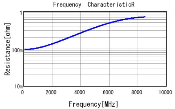
■ GJM0335C1E9R1BB01 R DCOV, 25degC
