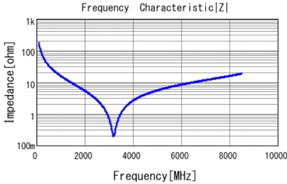
■ GJM0335C1E9R1BB01 |Z| DCOV, 25degC
