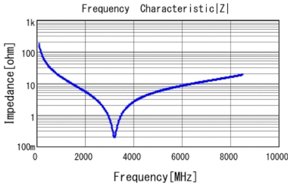
■ GJM0335C1E9R0DB01 |Z| DCOV, 25degC
