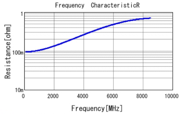
■ GJM0335C1E9R0DB01 R DCOV, 25degC
