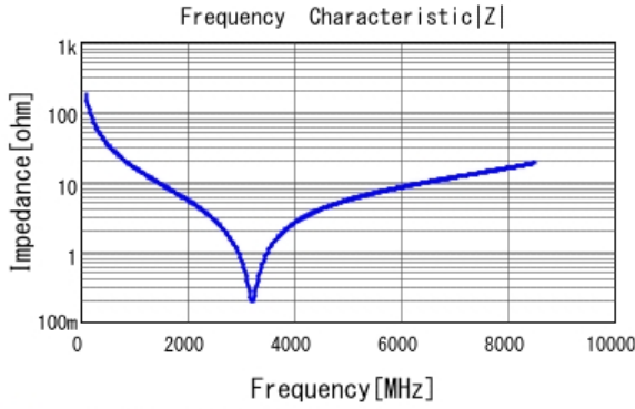
■ GJM0335C1E9R0CB01 |Z| DCOV, 25degC
