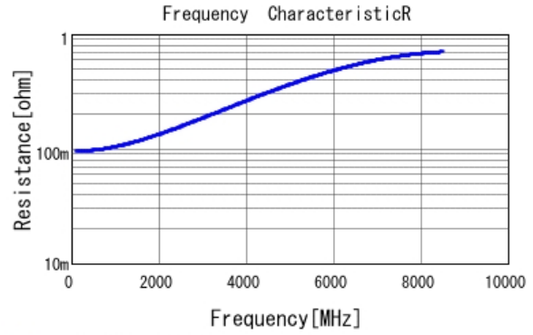
■ GJM0335C1E9R0CB01 R DCOV, 25degC
