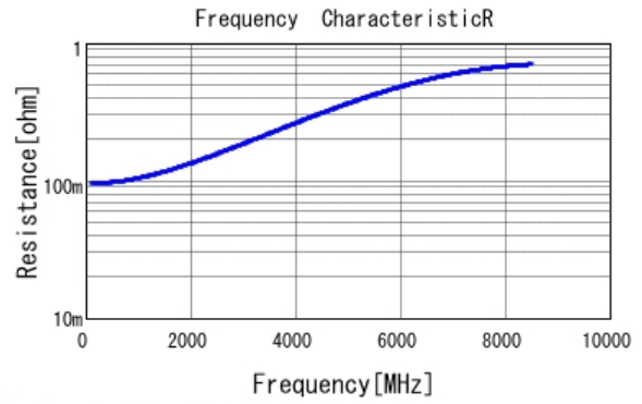
■ GJM0335C1E9R0BB01 R DCOV, 25degC
