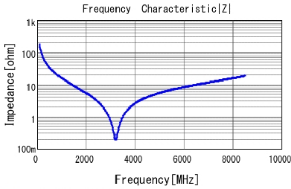
■ GJM0335C1E9R0BB01 |Z| DCOV, 25degC
