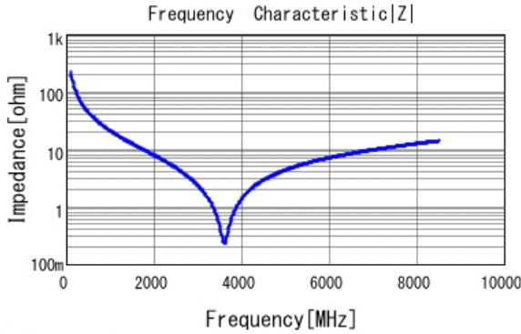
■ GJM0335C1E7R0WB01 |Z| DCOV, 25degC
