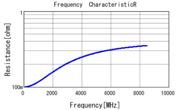
■ GJM0335C1E7R0WB01 R DCOV, 25degC
