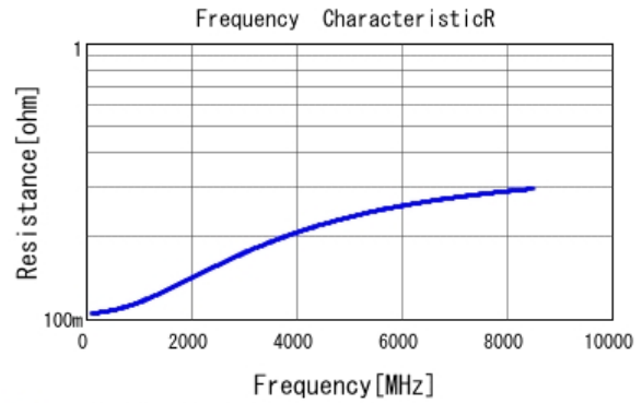
■ GJM0335C1E6R7BB01 R DCOV, 25degC
