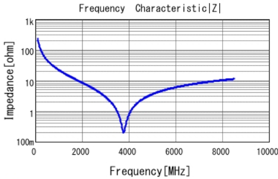
■ GJM0335C1E6R7BB01 |Z| DCOV, 25degC
