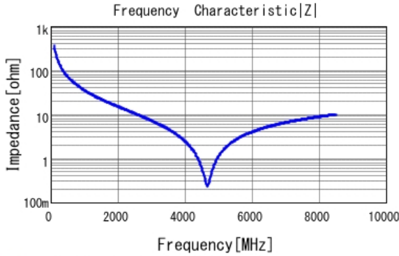
■ GJM0335C1E4R3WB01 |Z| DC0V, 25degC
