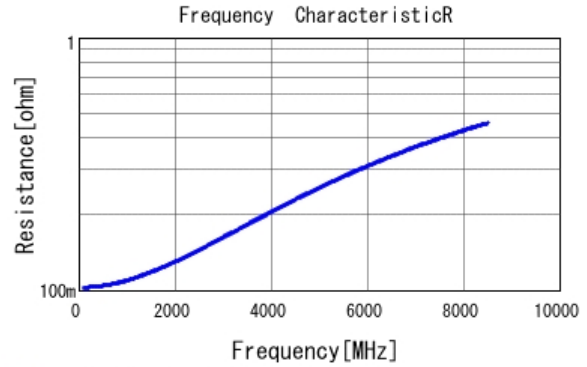
■ GJM0335C1E4R3WB01 R DC0V, 25degC
