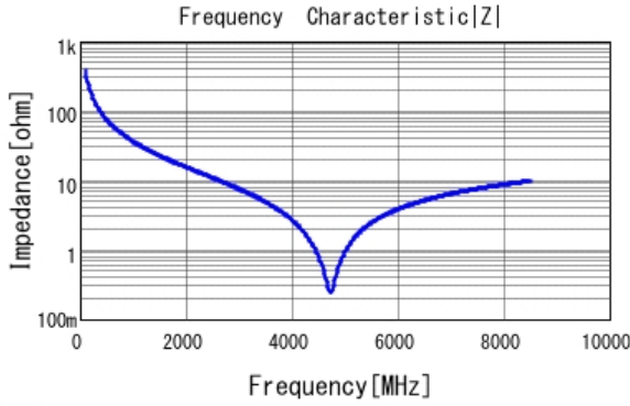
■ GJM0335C1E4R2WB01 |Z| DC0V, 25degC
