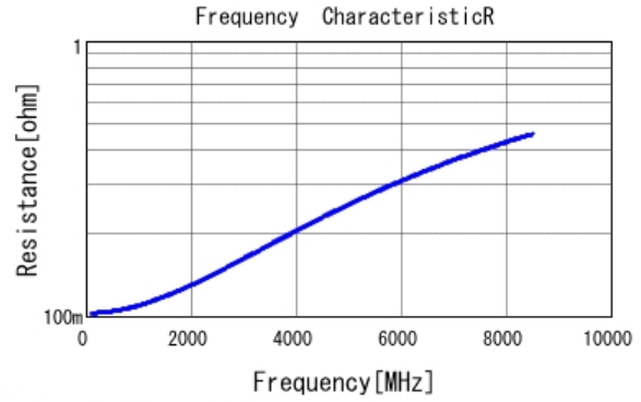
■ GJM0335C1E4R2WB01 R DC0V, 25degC
