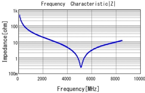
■ GJM0335C1E3R6BB01 |Z| DC0V, 25degC
