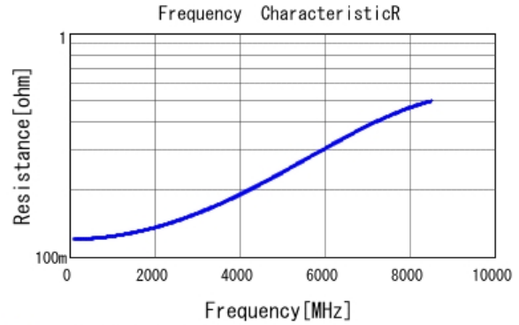
■ GJM0335C1E3R6BB01 R DC0V, 25degC
