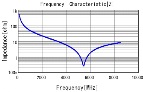
■ GJM0335C1E3R2WB01 |Z| DCOV, 25degC
