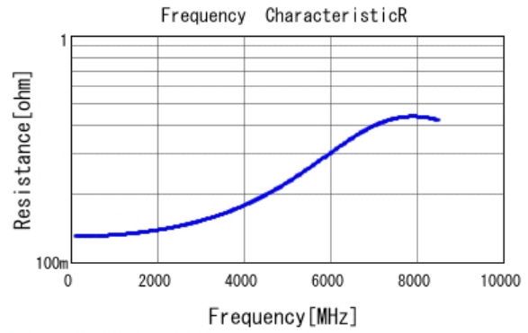
■ GJM0335C1E3R2WB01 R DCOV, 25degC
