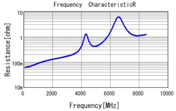
■ GJM0335C1E330JB01 R DCOV, 25degC
