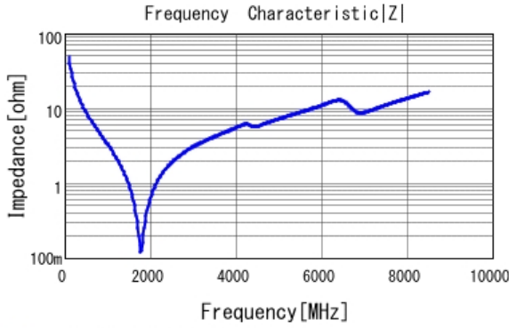
■ GJM0335C1E330JB01 |Z| DCOV, 25degC
