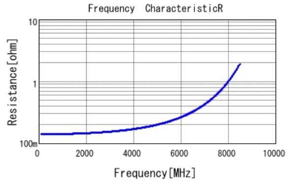
■ GJM0335C1E2R6WB01 R DC0V, 25degC
