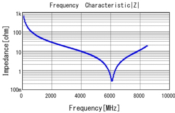
■ GJM0335C1E2R6WB01 |Z| DC0V, 25degC
