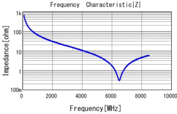
■ GJM0335C1E2R4WB01 |Z| DC0V, 25degC
