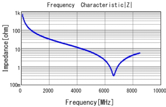
■ GJM0335C1E2R3CB01 |Z| DC0V, 25degC
