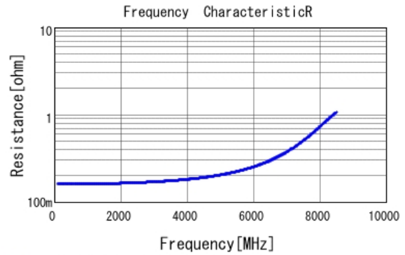
■ GJM0335C1E2R3CB01 R DC0V, 25degC
