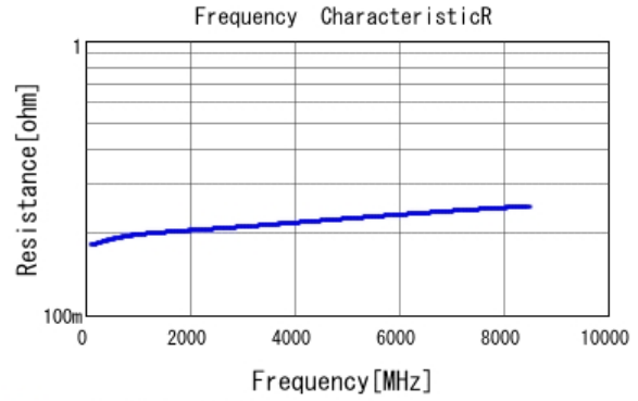
■ GJM0335C1E2R2CB01 R DC0V, 25degC
