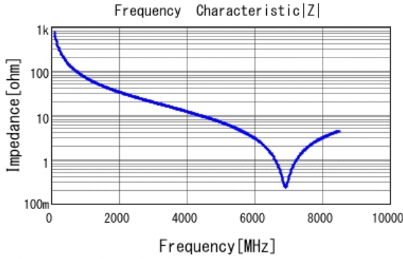
■ GJM0335C1E2R2CB01 |Z| DC0V, 25degC
