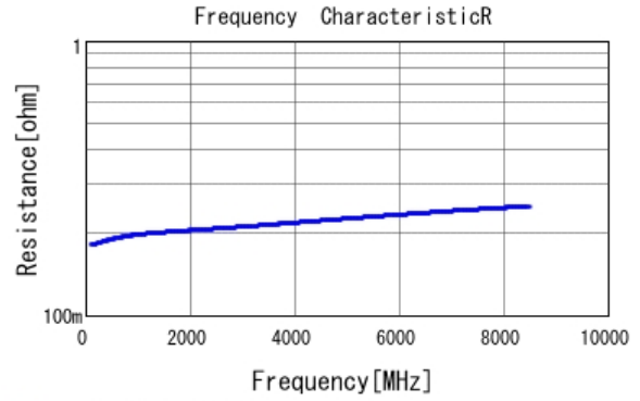
■ GJM0335C1E2R2BB01 R DC0V, 25degC
