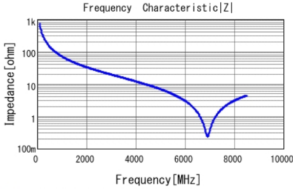
■ GJM0335C1E2R2BB01 |Z| DC0V, 25degC
