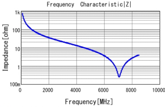
■ GJM0335C1E2R1WB01 |Z| DCOV, 25degC
