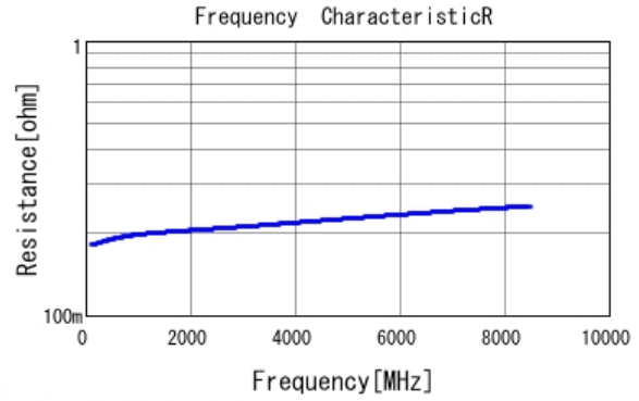
■ GJM0335C1E2R1WB01 R DCOV, 25degC
