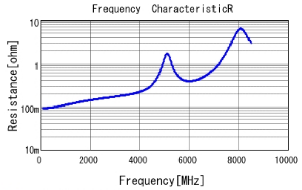
■ GJM0335C1E270JB01 R DC0V, 25degC
