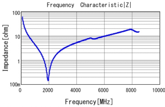
■ GJM0335C1E270JB01 |Z| DC0V, 25degC
