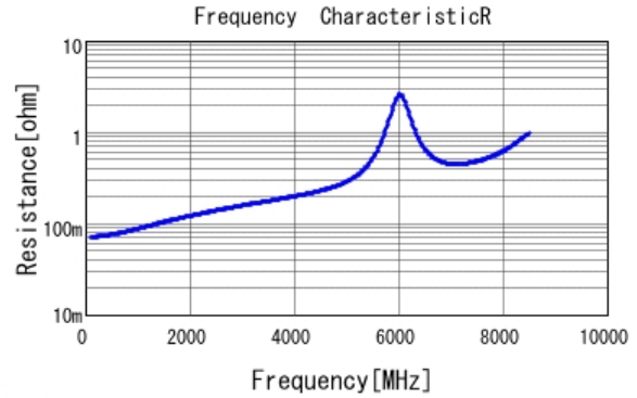
■ GJM0335C1E180GB01 R DC0V, 25degC
