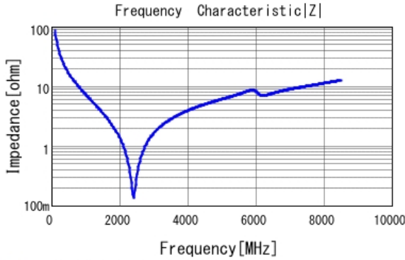
■ GJM0335C1E180GB01 |Z| DC0V, 25degC
