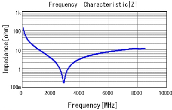
■ GJM0335C1E120GB01 |Z| DC0V, 25degC
