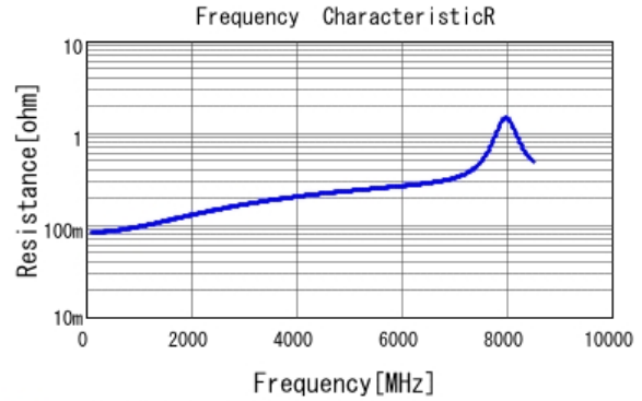
■ GJM0335C1E120GB01 R DC0V, 25degC
