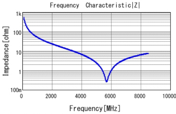
■ GJM0333C1E3R0CB01 |Z| DCOV, 20degC
