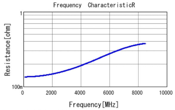
■ GJM0333C1E3R0CB01 R DCOV, 20degC
