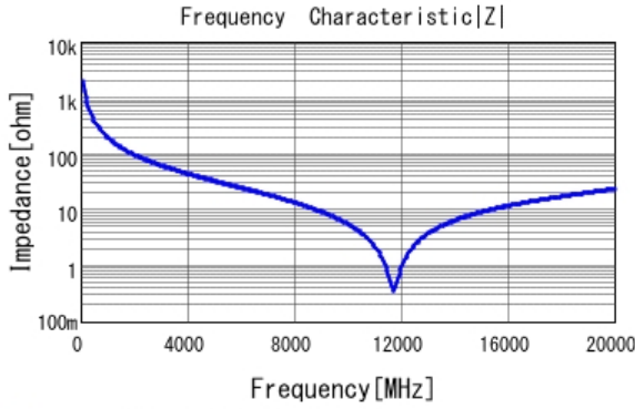
■ GJM0225C1ER80WB01 |Z| DCOV, 25degC
