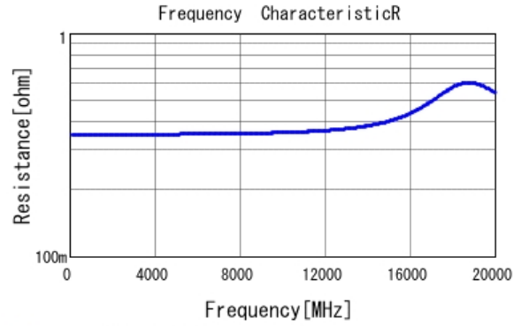
■ GJM0225C1ER80WB01 R DCOV, 25degC
