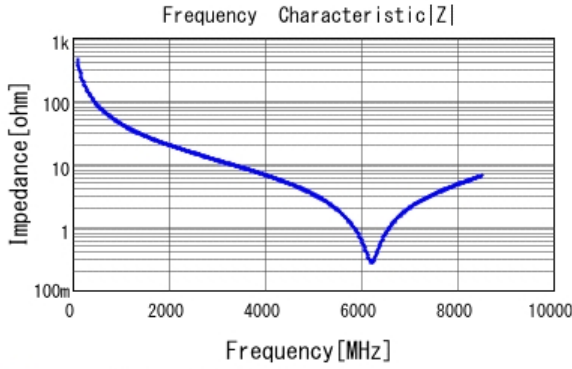
■ GJM0225C1E3R6WB01 |Z| DC0V, 25degC
