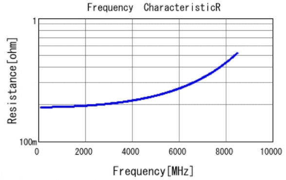
■ GJM0225C1E3R6WB01 R DC0V, 25degC
