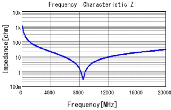
■ GJM0225C1E1R5WB01 |Z| DC0V, 25degC
