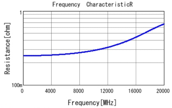
■ GJM0225C1E1R5WB01 R DC0V, 25degC
