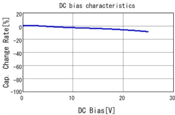
■ GJ431CC81E105KA01 C-DC bias capchange, 25.0degC, AC1.
