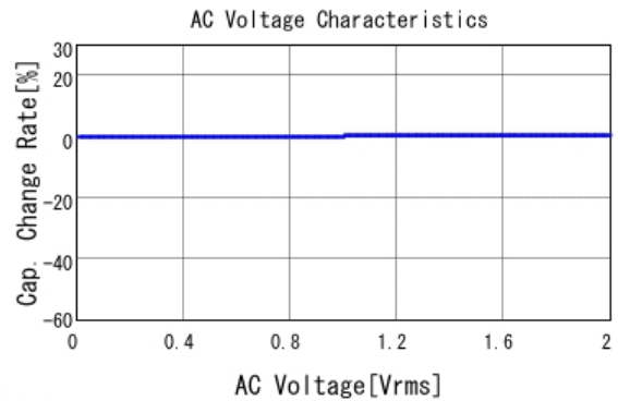
■ GJ431CC81E105KA01 C-AC Voltage capchange, DC0V, 25.0d
