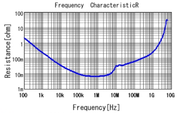
■ GJ431CC81E105KA01 R DC0V, 25degC
