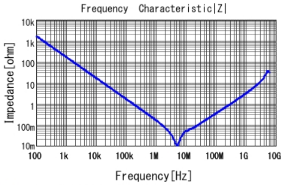
■ GJ431CC81E105KA01 |Z| DC0V, 25degC
