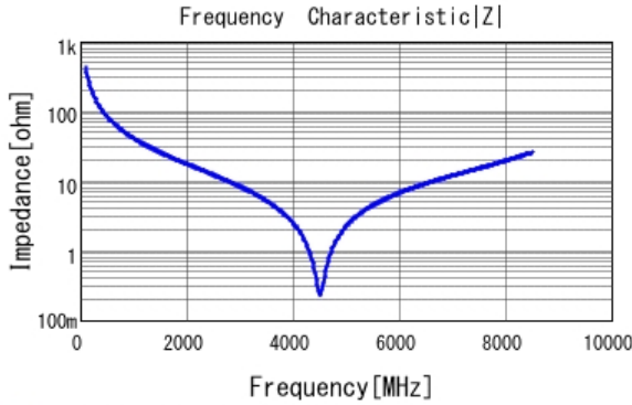
■ GCQ1555C1H3R7CB01 |Z| DC0V, 25degC
