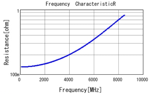
■ GCQ1555C1H3R7CB01 R DC0V, 25degC
