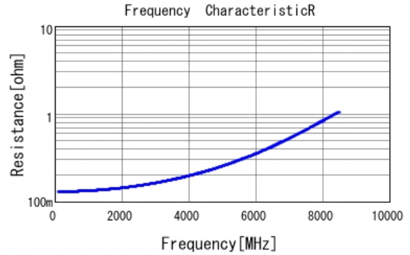
■ GCQ1555C1H3R2BB01 R DC0V, 25degC
