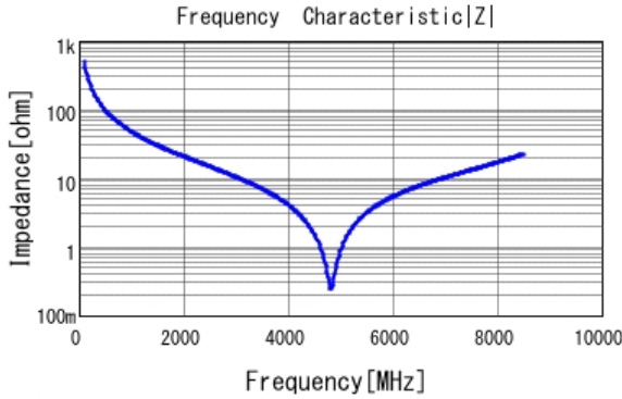
■ GCQ1555C1H3R2BB01 |Z| DC0V, 25degC
