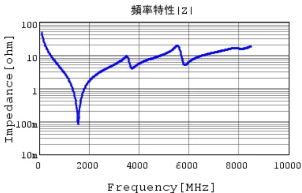
GCQ1555C1H330JB01 |Z| DCOV, 25degC
