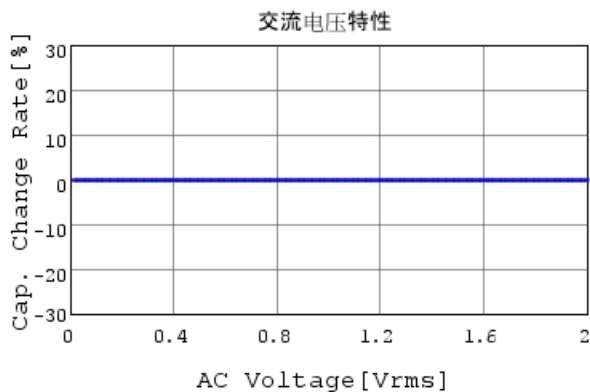
GCQ1555C1H330JB01 C-AC Voltage capchange, DC
