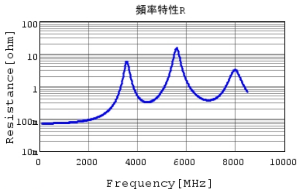
GCQ1555C1H330JB01 R DCOV, 25degC
