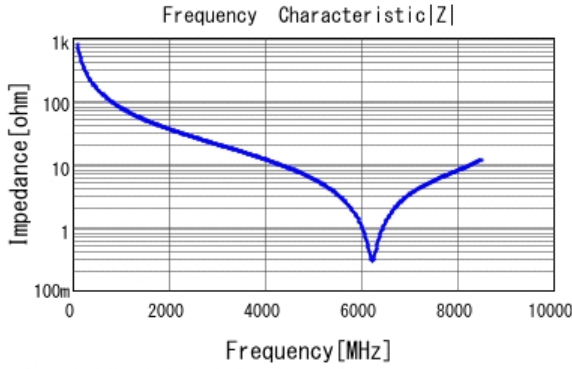
■ GCQ1555C1H2R0WB01 |Z| DCOV, 25degC
