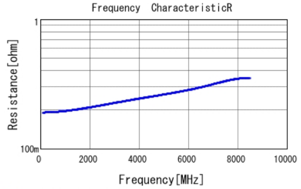
■ GCQ1555C1H2R0WB01 R DCOV, 25degC
